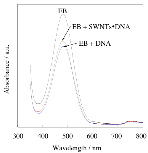
Supplementary Fig. 3 UV-Vis absorption spectra of EB, EB+DNA and EB+SWNTs•DNA complexes in 50 mmol dm -3 phosphate buffered saline (pH 6.98) at 25 °C: [EB] = 50.7 μmol dm -3 , [DNA] = 1.33 mmol dm -3 (base unit), [SWNT] = 2.97 μg dm -3 .
